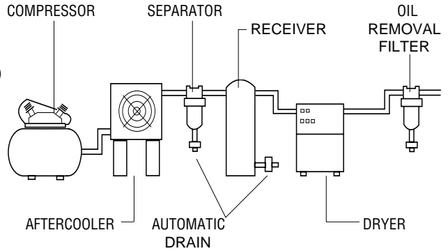
TYPICAL COMPRESSED AIR SYSTEM
